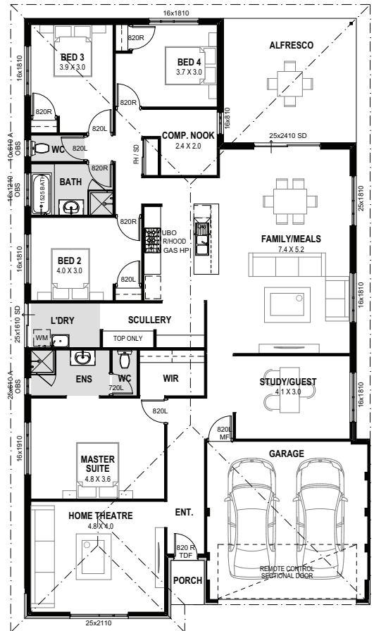
Floor Plan
